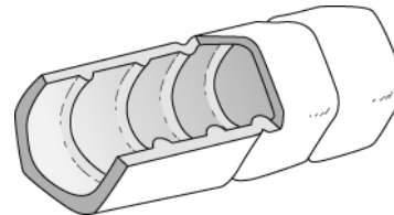
Xylem cells carry water.
